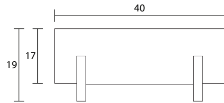
Sideview/Frontview
